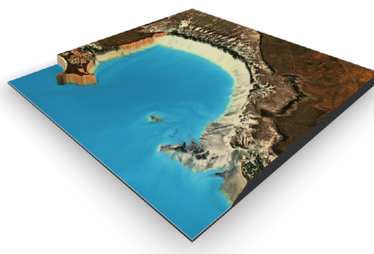
Figure 11.4 National Intertidal Digital Elevation Model
