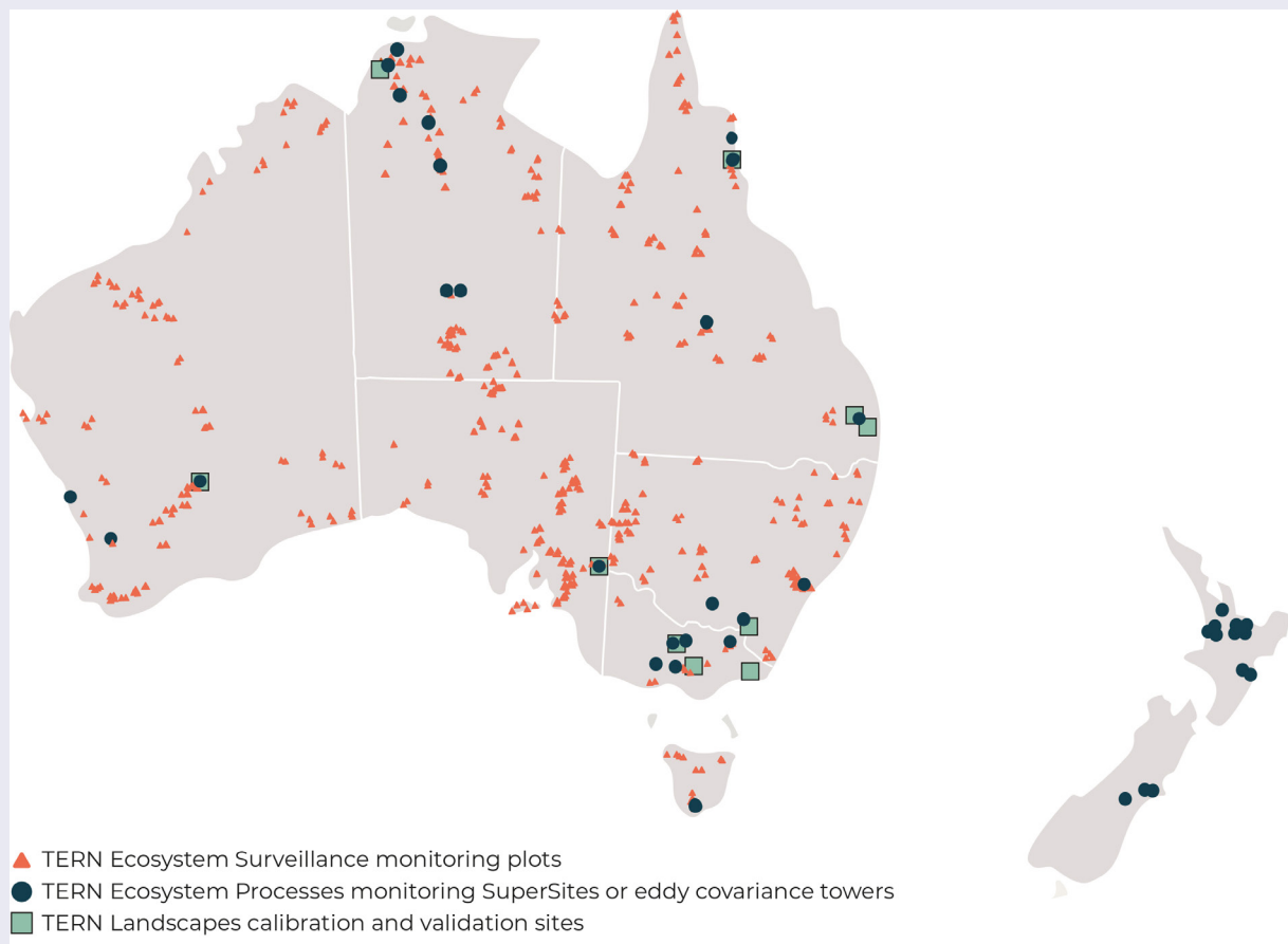
Figure 12.1 TERN sites
