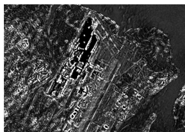
Euclidean difference
