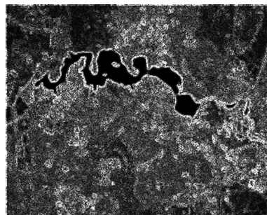
Euclidean difference
