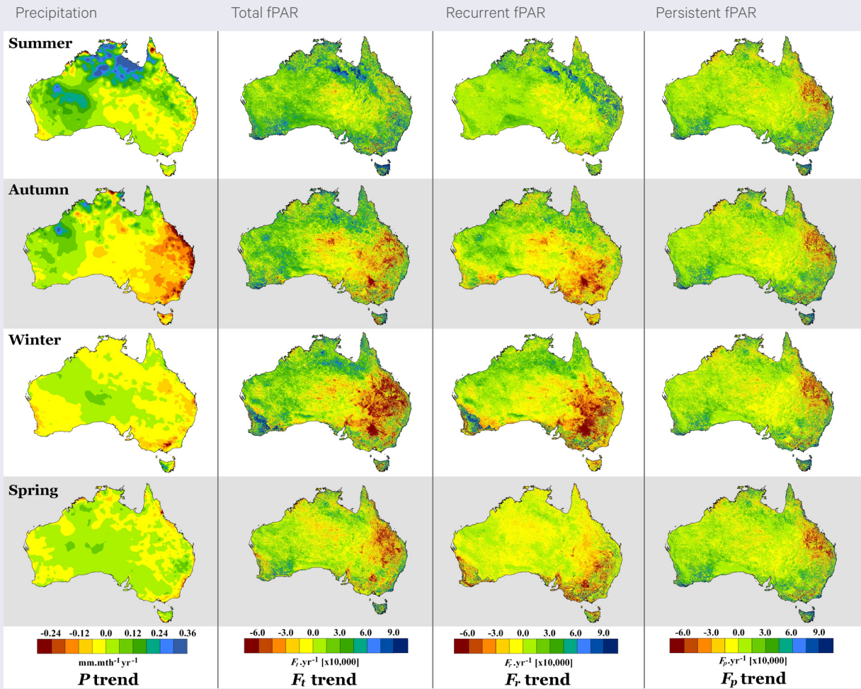
Figure 8.6 Seasonal trends 1981–2006
