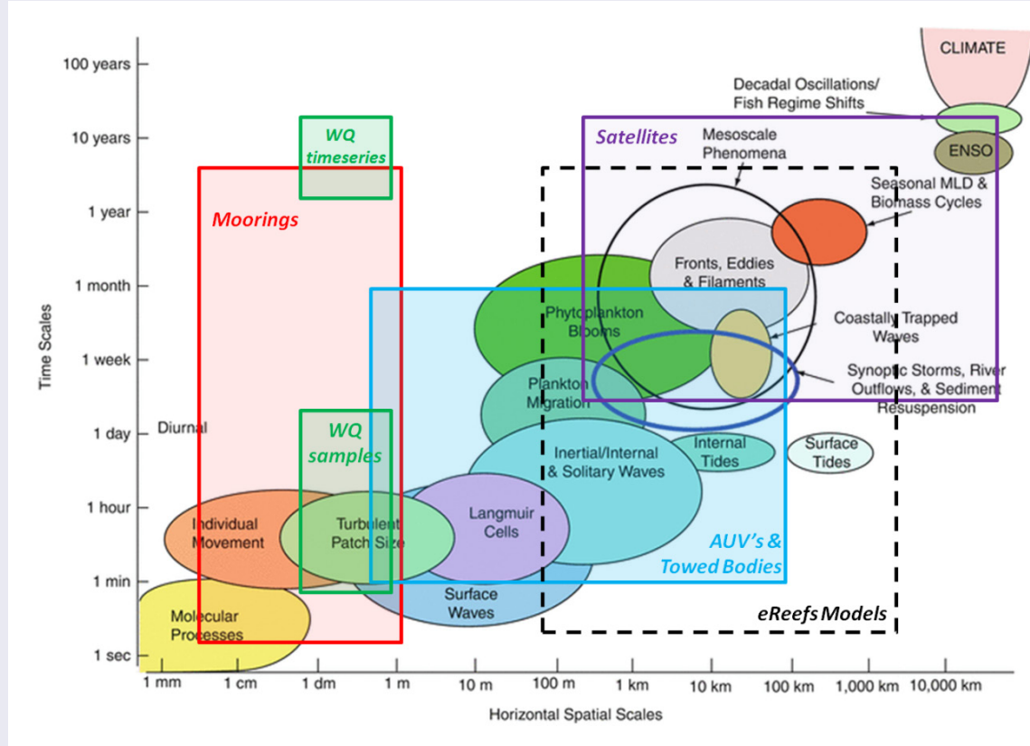
Figure 14.8 Temporal and spatial scales of GBR processes and observations
